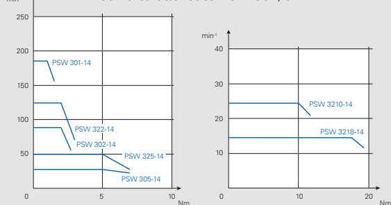
Curva caratteristica PSW 30x/32x-14
