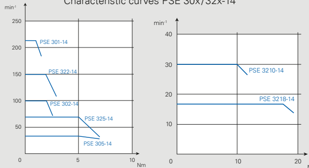
Characteristic curves PSE 30x/32x-14
